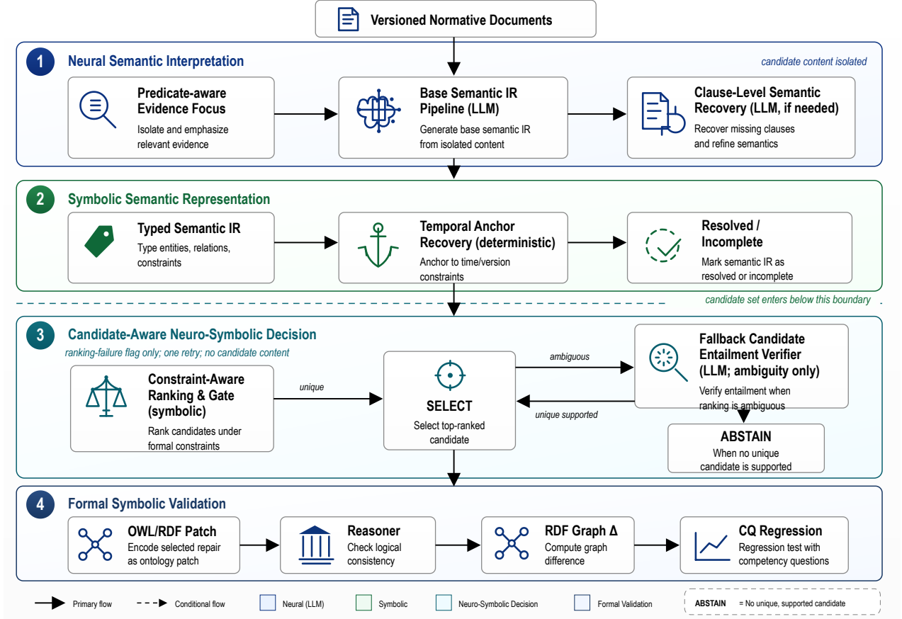
Figure 1: Overall evidence-constrained neuro-symbolic architecture of ECR-REPAIR. Semantic IR is the neural-to-symbolic interface; the candidate set becomes visible only in the candidate-aware decision layer. The Fallback Candidate Entailment Verifier is triggered only when symbolic ranking is ambiguous, and the dashed feedback path carries only a content-free ranking-failure flag.
