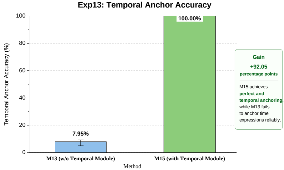
Figure X. Temporal anchor accuracy comparison (Exp13). M13 without temporal modeling fails to resolve temporal context in most cases, while M15 with temporal modeling achieves perfect accuracy.
